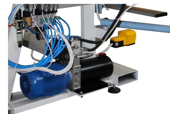
Pompa idraulica per taglio e avanzamento foratrice Hydraulic pump for cutting and perforating machine advance
